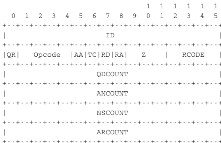
Figure 3.3: DNS header
