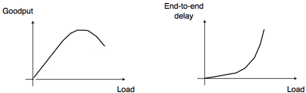
Figure 2.66: Network congestion
