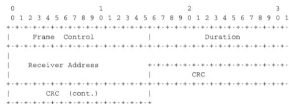
Figure 3.97: IEEE 802.11 ACK and CTS frames
