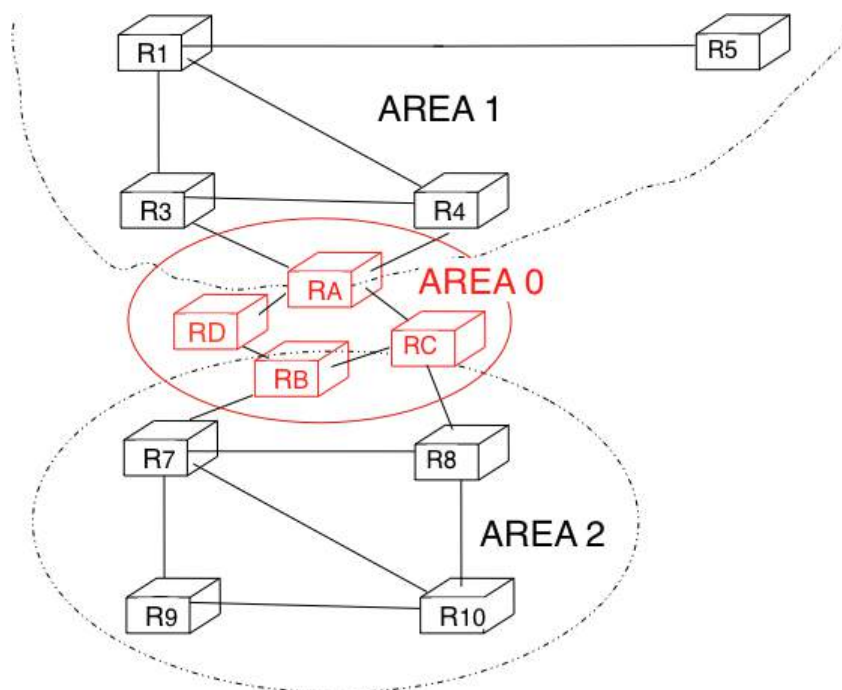
Figure 3.62: OSPF areas
