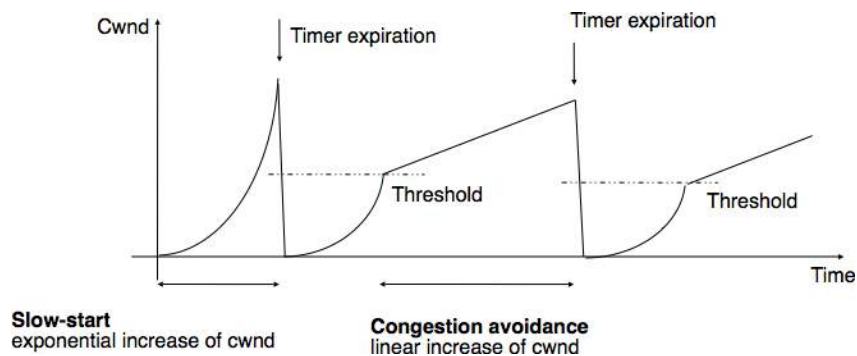
Figure 3.37: Evaluation of the TCP congestion window with severe congestion
