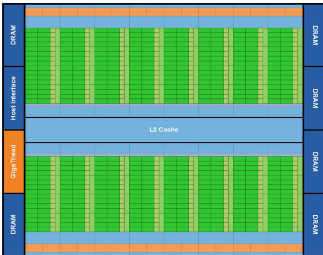
Figure 38. A schematic of the Fermi architecture. Color code: orange - scheduling and dispatch; green - execution; light blue – registers and caches. The co-processor is made up of a collection of 16 Stream Multiprocessors (SMs). Details of an SM are provided in Figure 44. Credit: Nvidia.
