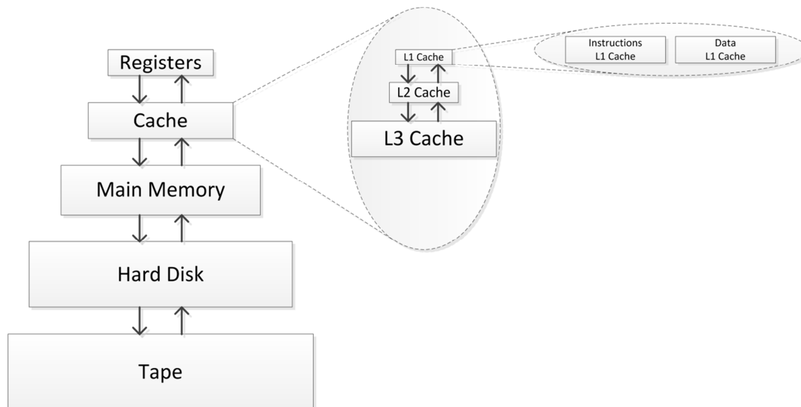
Figure 13. The memory hierarchy. From up to down: more memory, longer access times. In general, this is a true hierarchy: data stored at a higher level is also stored at a lower level. Of these storage spaces, only the registers and caches are on the CPU. Of any two blocks in this figure, the bigger one suggests a larger amount of memory associated with that level. The relative size of blocks though is not proportional to the relative size of the actual memories. For instance, a relatively recent Intel processor, Intel Core i3-2100, has a processor with two cores; each
