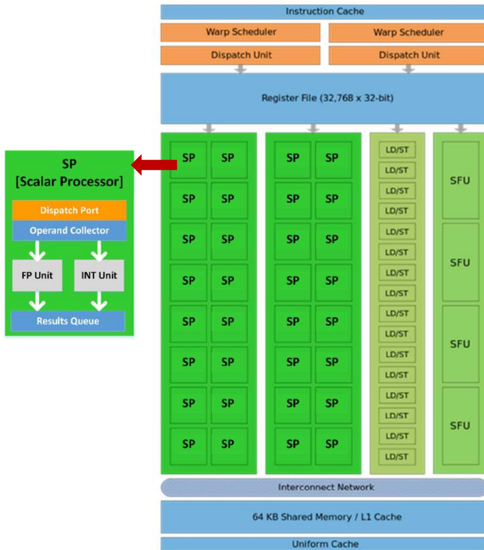
Figure 44. Architecture of a Stream Multiprocessor (SM). Fermi has four functional units: two blocks of 16 SPs each, a group of four SFUs, and a set of 16 load/store units. Color code: orange - scheduling and dispatch; green - execution; light blue - registers and caches. Credit: Nvidia.
