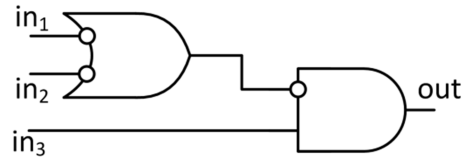
Figure 4. Logic block that implements the requested truth table. Inverters are represented by circles ○ applied to signals moving down the bus.
