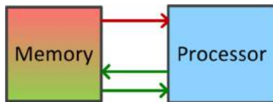
Figure 25. Schematic of early system architecture. Blue is used to indicate a hardware asset that processes information. Green is used for data flow. Red is used for commands/instructions that the processor is expected to honor. The memory shows a mixture of green and red as it stores both instructions and data.
