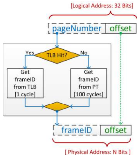
Figure 21. Schematic of the page translation process that involves the TLB. The latency is two orders of magnitude higher upon a TLB miss.
