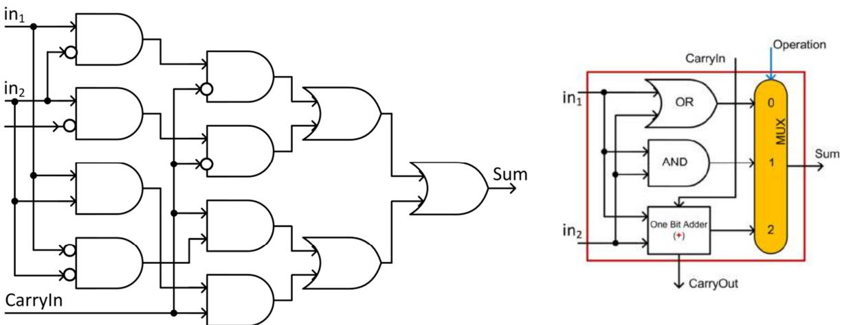
Figure 7. Hardware implementation in terms of gates to support the logic required to produce the Sum signal given the three inputs \text{in}_1 , \text{in}_2 , and CarryIn (Left). This logical unit, augmented with the logical unit that produces CarryOut (Figure 6, right), is packaged as in Figure 6, left, and then combined with a MUX to produce a one bit ALU complex combinational block (Right) capable of performing AND, OR, and addition.
